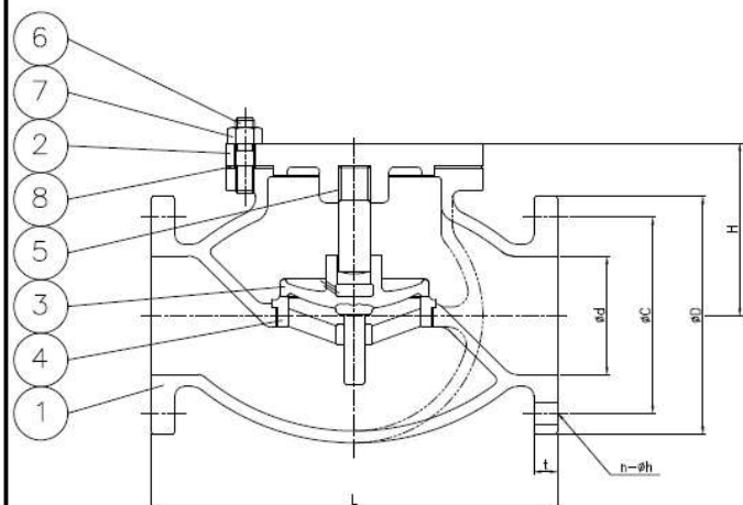
LIFT CHECK GLOBE VALVE
